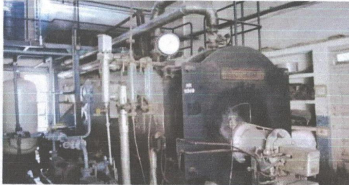
Photo: Oil Fired Fire Tube Boiler Used in Nandan Dairy Plant
